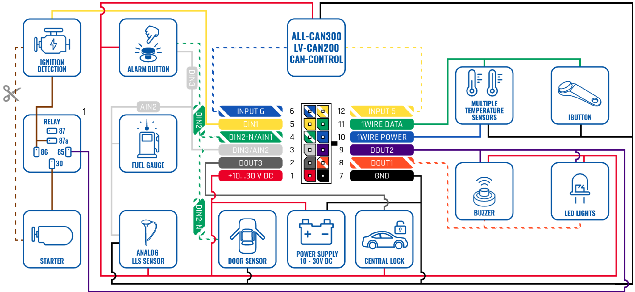
Figure 3 FMC230 Wiring scheme
